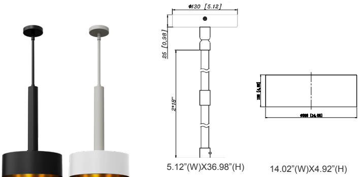
CMC2XL-MCT-DD-BK+CMC-SRK-218-5C-BK+CMC2-PS14-BG CMC2XL-MCT-DD-WH+CMC-SRK-218-5C-WH+CMC2-PS14-WG
