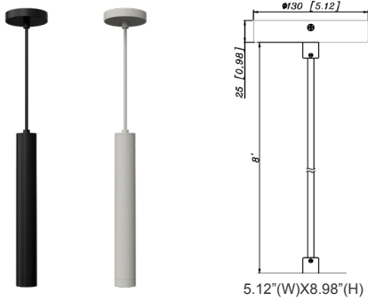
CMC2XL-MCT-DD-BK+CMC-CS-8FT-BK CMC2XL-MCT-DD-WH+CMC-CS-8FT-WH
