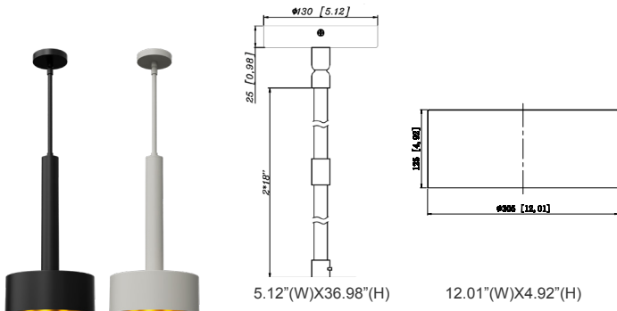
CMC2XL-MCT-DD-BK+CMC-SRK-218-5C-BK+CMC2-PS12-BG CMC2XL-MCT-DD-WH+CMC-SRK-218-5C-BK+CMC2-PS12-WG
